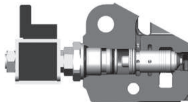
BEN – Electrically controlled pump-unloading function.
